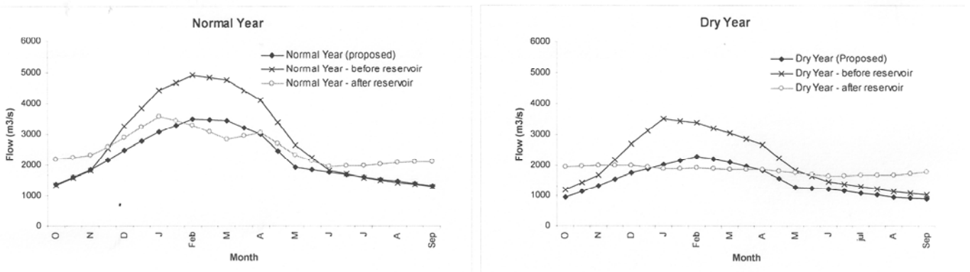
Figure 2 - Environmental flow hydrograms required for: (I) normal year and (II) dry year
