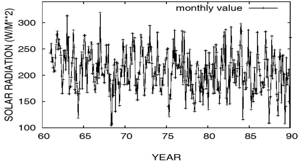
Figure 9. Monthly values of solar radiation ( W/m^2 ) in Salvador, Bahia, Brazil, in the period 1961-1990.
