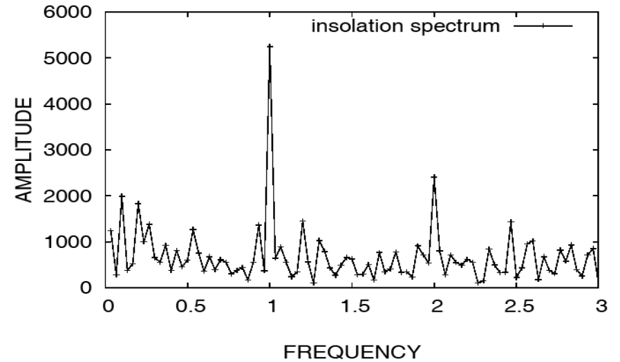
Figure 10. Solar radiation spectrum in Salvador, Bahia, Brazil, in the period 1961-1990.
