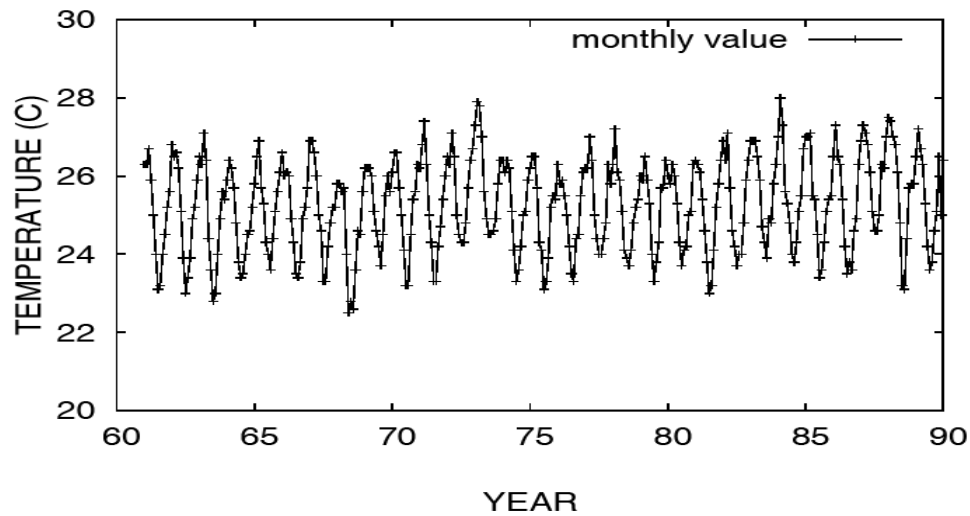
Figure 3. Monthly values of average temperature (°C) in Salvador, Bahia, Brazil, in the period 1961-1990.
