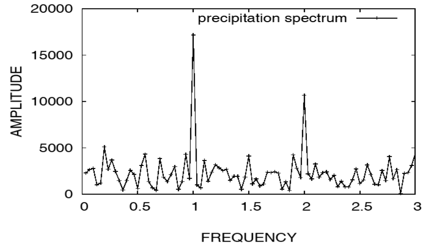
Figure 2. Precipitation spectrum in Salvador, Bahia, Brazil, in the period 1961-1990.
