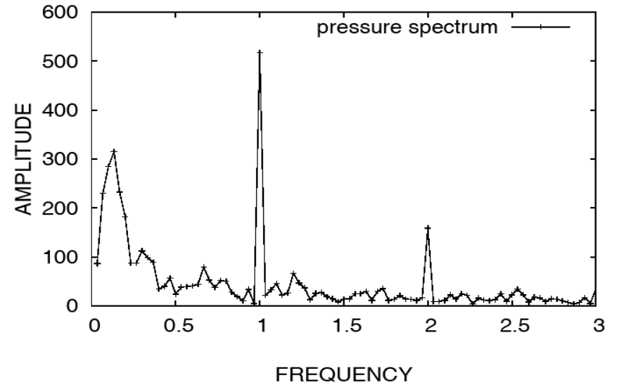
Figure 6. Pressure spectrum in Salvador, Bahia, Brazil, in the period 1961-1990.
