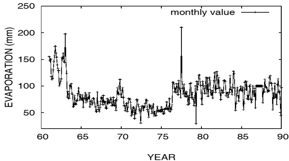
Figure 15. Monthly values of evaporation ( \text{mm} ) in Salvador, Bahia, Brazil, in the period 1961-1990.
