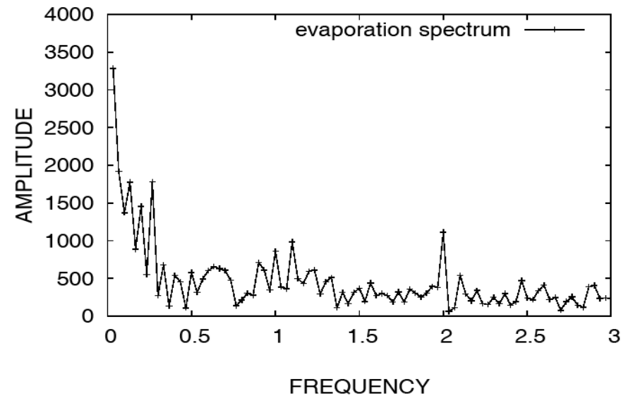
Figure 16. Evaporation spectrum in Salvador, Bahia, Brazil, in the period 1961-1990.
