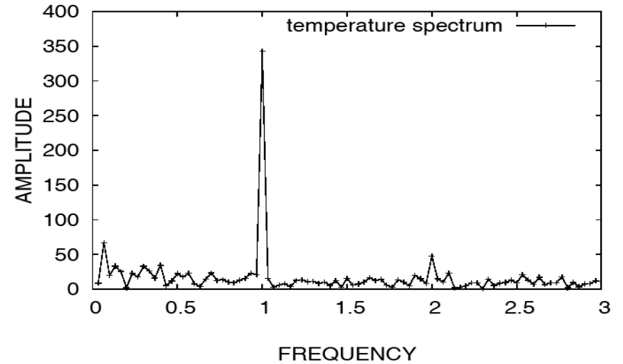
Figure 14. Maximum temperature spectrum in Salvador, Bahia, Brazil, in the period 1961-1990.
