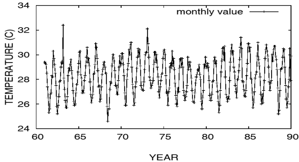
Figure 13. Monthly values of maximum temperature ( ^{\circ}\text{C} ) in Salvador, Bahia, Brazil, in the period 1961-1990.
