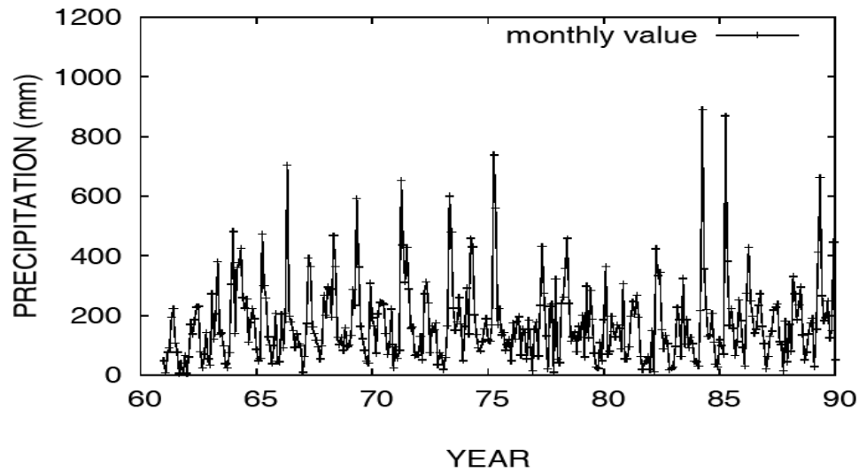
Figure 1. Monthly values of precipitation (mm) in Salvador, Bahia, Brazil, in the period 1961-1990.
