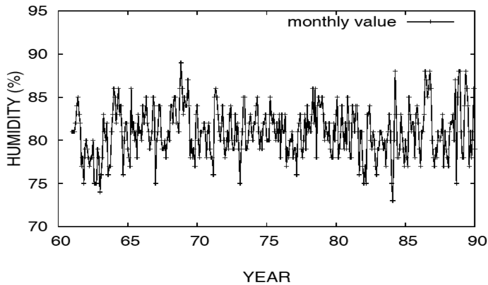
Figure 7. Monthly values of humidity (%) in Salvador, Bahia, Brazil, in the period 1961-1990.
