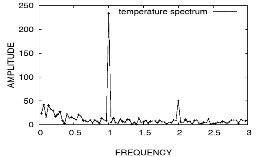
Figure 12. Minimum temperature spectrum in Salvador, Bahia, Brazil, in the period 1961-1990.
