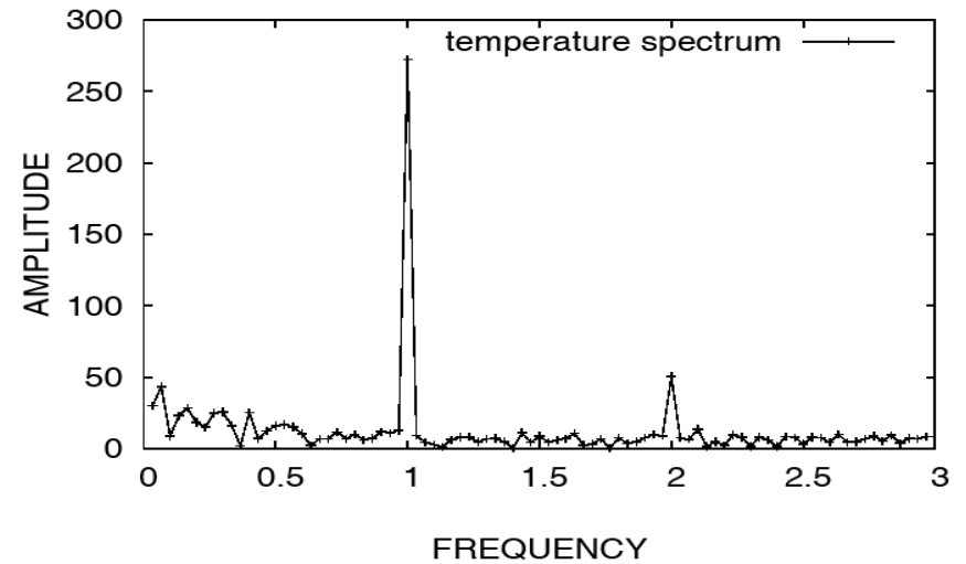
Figure 4. Average temperature spectrum in Salvador, Bahia, Brazil, in the period 1961-1990.
