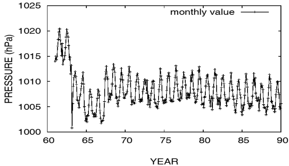
Figure 5. Monthly values of pressure (hPa) in Salvador, Bahia, Brazil, in the period 1961-1990.
