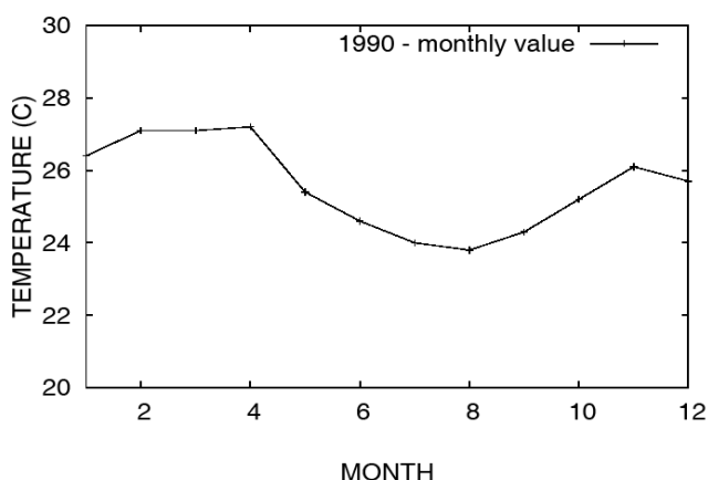
Figure 18. Monthly values of average temperature (°C) in Salvador, Bahia, Brazil, for the year 1990.
