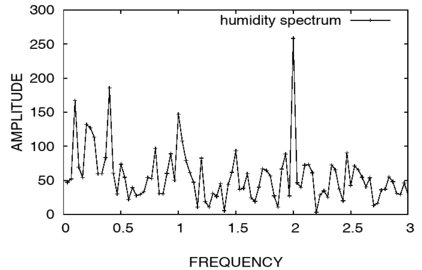
Figure 8. Humidity spectrum in Salvador, Bahia, Brazil, in the period 1961-1990.
