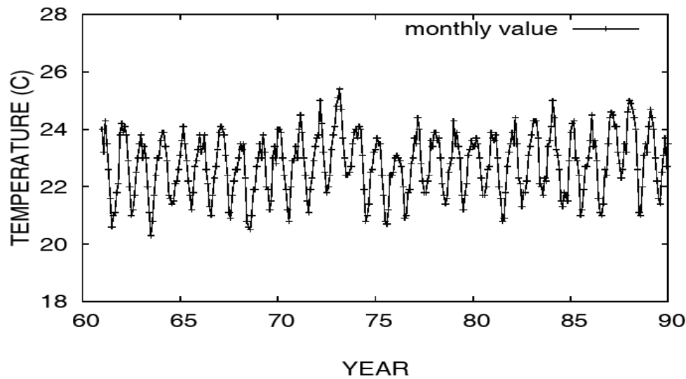
Figure 11. Monthly values of minimum temperature ( ^{\circ}C ) in Salvador, Bahia, Brazil, in the period 1961-1990.
