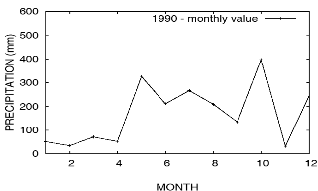
Figure 17. Monthly values of precipitation (mm) in Salvador, Bahia, Brazil, for the year 1990.
